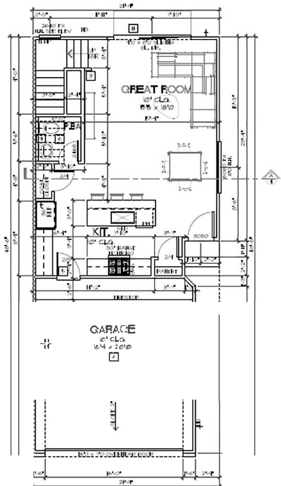
First Level
