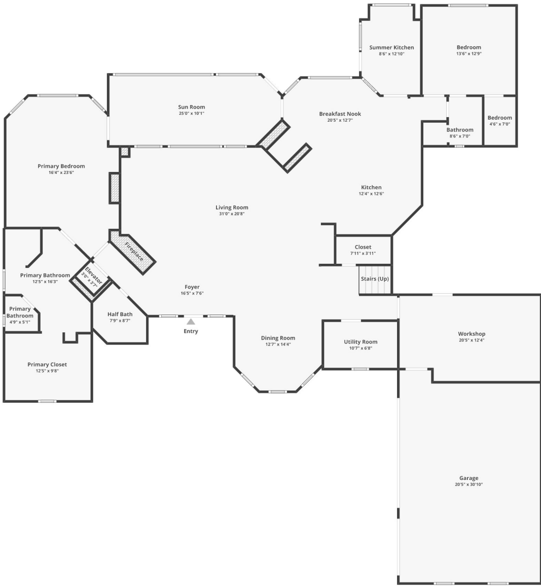
FLOOR 1
