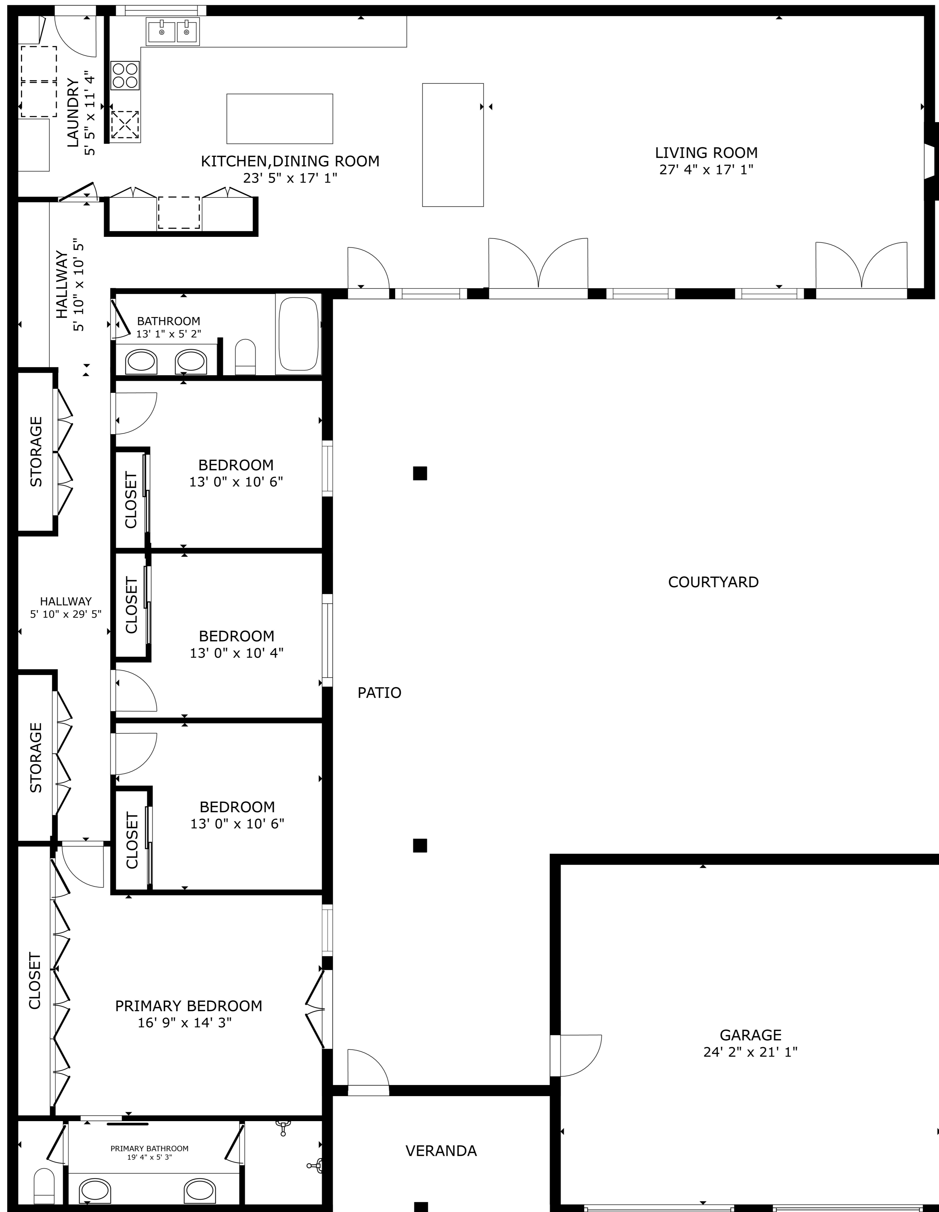
FLOOR PLAN
